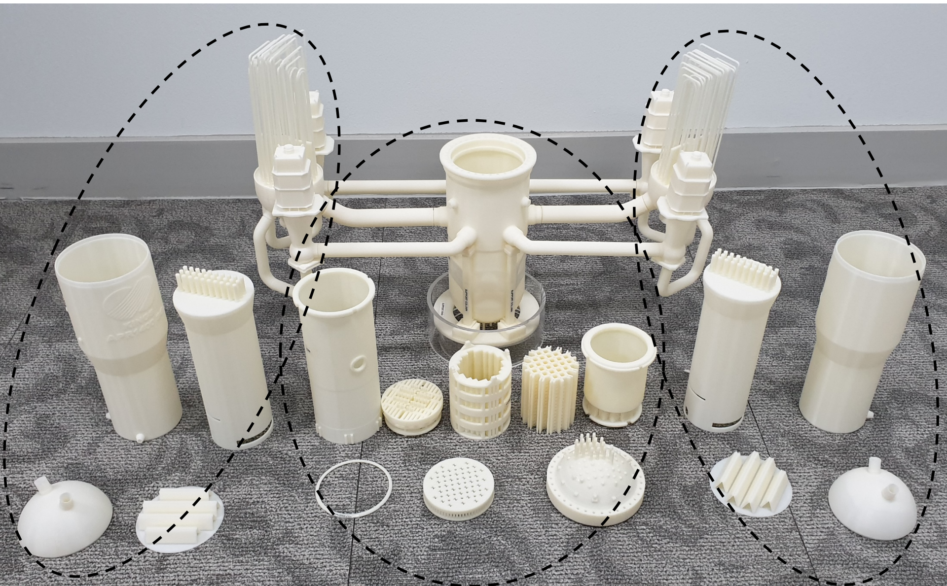
Steam Generator components
